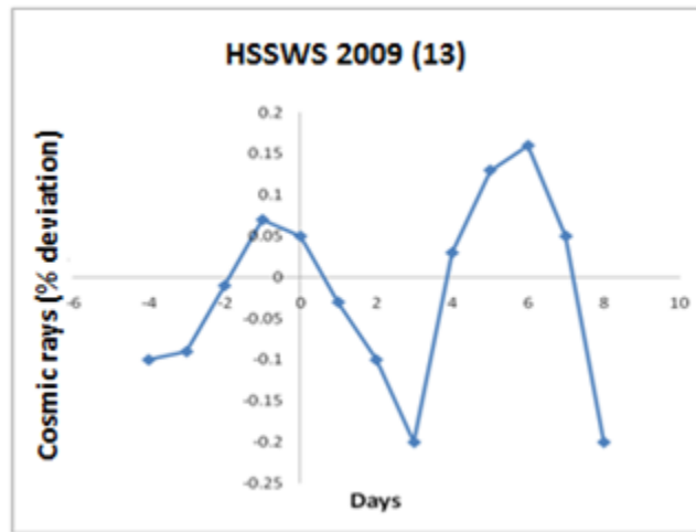
Figure 1.1: The result of chree analysis of superposed epoch method from -4 to 8 days with respect to zero epoch days for the year of 2009.the percent deviation of the daily mean cosmic ray intensity (Oulu neutrons) for a number
