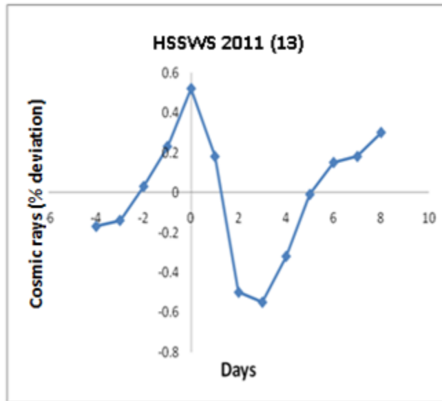
Figure 1.3: Same as figure 1.1 but for the year 2011
